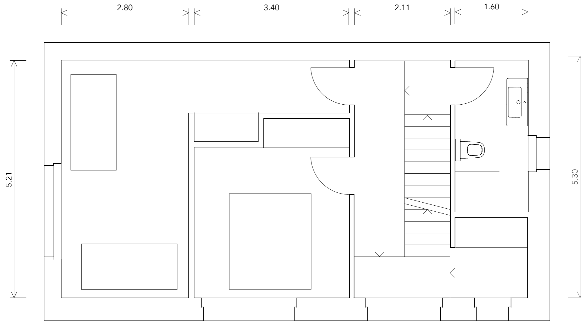
Schlafzimmer 1 Bedroom 1 19.50m 2
